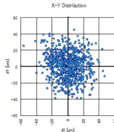
Figure 13: X Y Pickup Position Repeatability Results from Test 2
