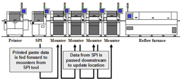
Figure 14: Theoretical SMT Line utilizing Adaptive Process Control
