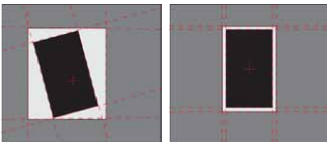
Figure 11: Component size to pocket ratio is critical to control for accurate pick
