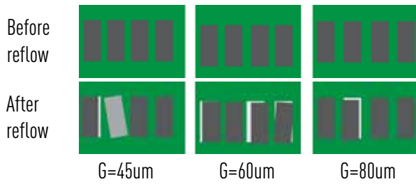
Figure 10 Image of Solder Bridge Test Results
