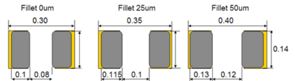
Figure 8: Substrate Pad and Stencil Screen Apertures Conditions
