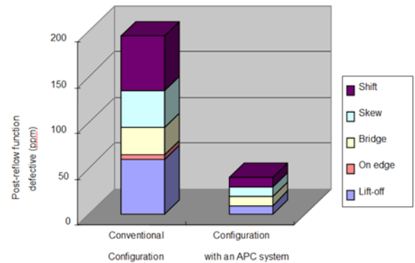
Figure 17: Post-reflow Defect Reduction Effects with Adaptive Process Control
