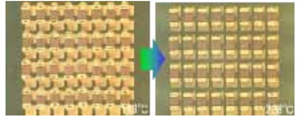
Figure 16: APC-controlled Placements with Chips Located on Solder Deposit (before and after reflow)
