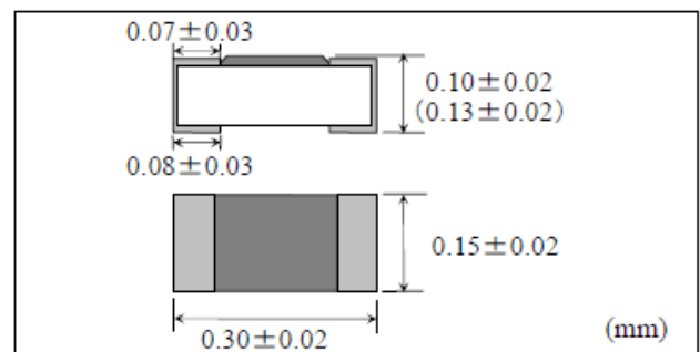
Figure 2: Tentative 03015M Component Dimensions
