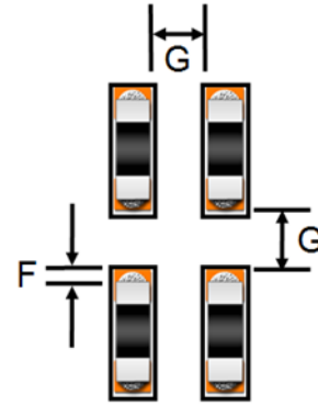
Figure 7: Fillet (F) and Gap (G) need to be optimized
