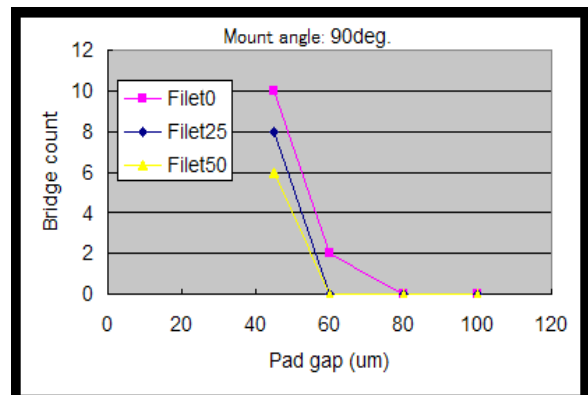
Figure 9: Graphical Results of Solder Bridge Test
