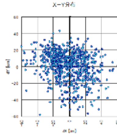
Figure 12: X Y Pickup Position Repeatability Results from Test 1
