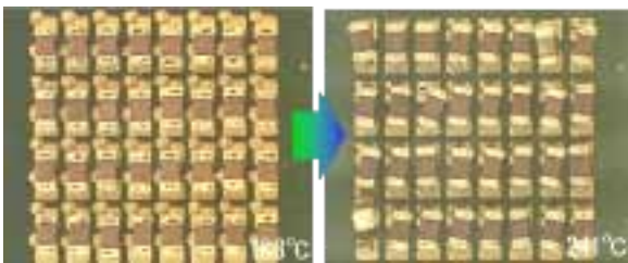
Figure 15: Traditional Placements with Chips Located on Pads (before and after reflow)
