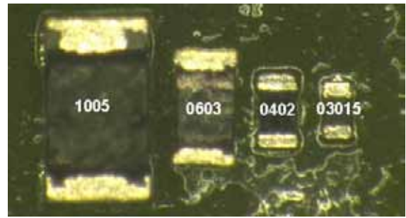
Figure 1: Passive Component Size Comparisons (0402 represents 01005 standard)
